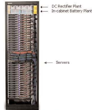
Figure 7: Cluster Server Cabinet and 20kW d 2 ups Uninterruptible DC Power Plant
