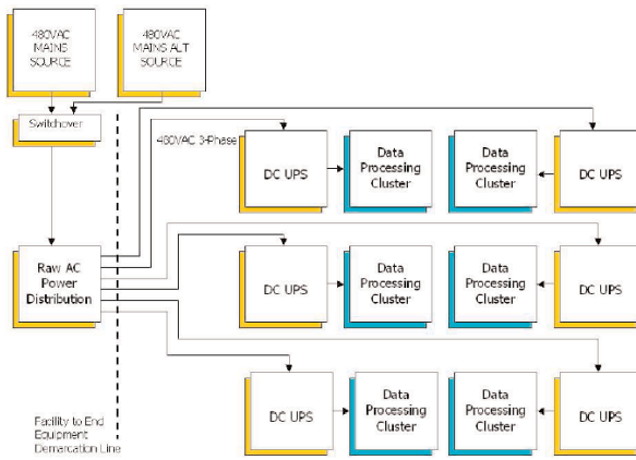
Figure 4: Distributed DC UPS
