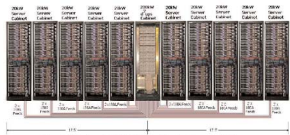
Figure 6: Distributed DC UPS Physical Realization - 200kW Cluster
