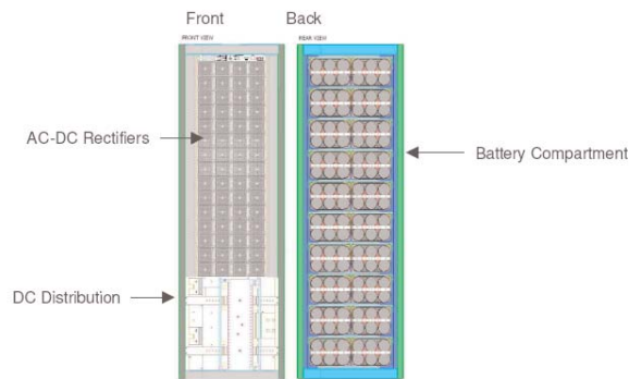
Figure 5: 200kW DC UPS for Distributed DC UPS Architecture
