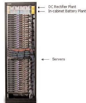
Figure 7: Cluster Server Cabinet and 20kW d 2 ups Uninterruptible DC Power Plant
